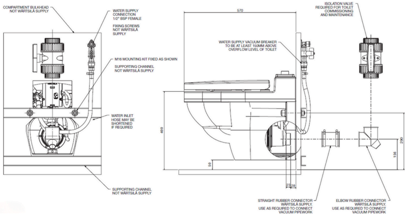
Fig. 1 Installation data and interface requirements
